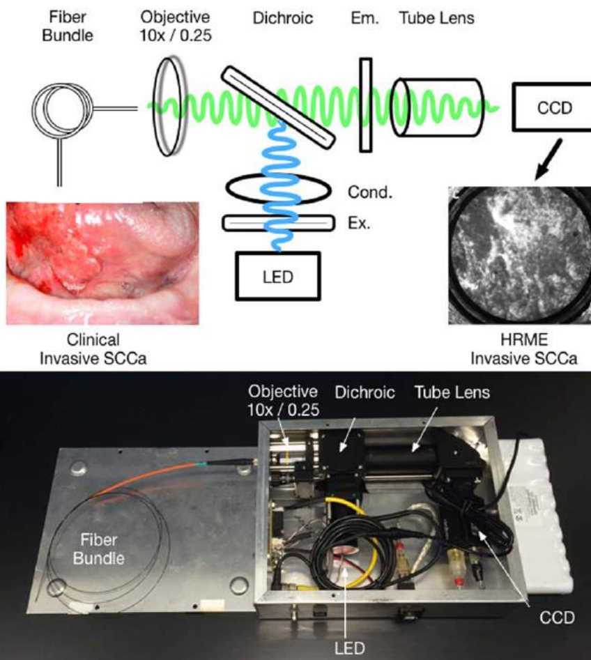
Fig. 1. The high-resolution microendoscope, shown in schematic (A) and fully assembled (B). Note that the associated computer tablet/viewing screen is not shown. CCD = Charge-coupled device; Cond = Condenser Lens; Ex = Excitation Filter; Em = Emission Filter; HRME = High Resolution Microendoscopy; LED = Light emitting diode; SCCa = squamous cell carcinoma.
