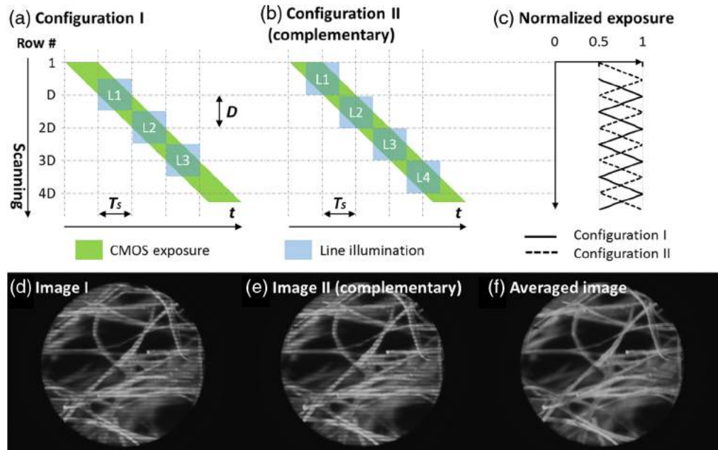
Fig. 2 Synchronization of the CMOS and DLP and construction of a confocal image by averaging two complementary images. Imaging configuration I in (a) shows the spatiotemporal coordination of the DLP illumination lines with the CMOS rolling shutter aperture; the discrete nature of DLP scanning combined with the continuous sequential readout of CMOS rows introduces nonuniform exposure among the rows, as revealed in configuration I in (c) and the corresponding image (d). A complementary image (e) can be acquired by shifting the exposure distribution by D/2 in configuration II in (b). A confocal image without illumination artifacts is then constructed by averaging two complementary frames, as shown in (d), (e), and (f). Lens paper was imaged as a target. D , number of rows in the detection aperture; T_s , CMOS exposure time.
