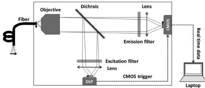
Fig. 1 Schematic of the line scanning confocal HRME platform. Solid arrows show directions of scanning on the DLP, CMOS, and fiber surface; dashed arrows show the data flow between the DLP, camera, and laptop. The solid box indicates the optical system enclosure.
