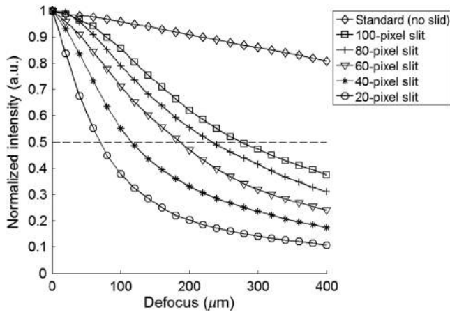
Fig. 3 Optical sectioning profiles of the standard HRME (no slit) and confocal HRME (20, 40, 60, 80, and 100-pixel slit). The line scanning confocal configurations significantly improve the axial resolution of the standard HRME. As the slit size increases, the axial performance transits from the confocal to nonconfocal regime. A 20-pixel slit on the CMOS sensor is about 16.5 \mu\text{m} on the fiber surface.
