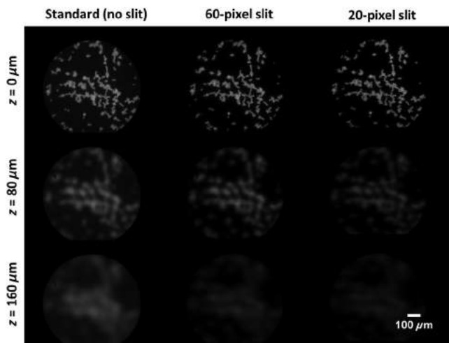
Fig. 4 2-D phantom images with varied slit widths. Images acquired at a defocus of 0, 80, and 160 \mu\text{m} are shown for the standard HRME and two confocal configurations (60-pixel and 20-pixel slits). Compared with the image at 0 \mu\text{m} , the corresponding image at 80 and 160 \mu\text{m} revealed signal loss and indicated rejection of background signal. The signal loss was most significant using the 20-pixel slit, suggesting that a smaller detection slit in the confocal configuration improves optical sectioning capability.
