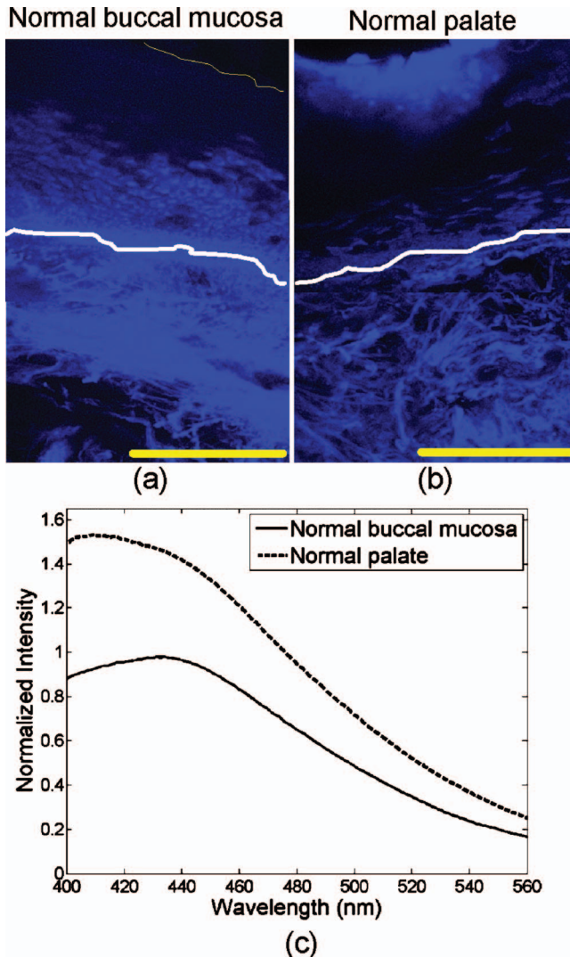
Fig. 3 (a) and (b) Fluorescence confocal images and (c) measured fluorescence spectra at UV excitation, showing changes in autofluorescence patterns due to anatomic site variation. (a) Normal buccal mucosa; and (b) normal palate. In (a) and (b), the white lines represent the basement membrane and the yellow lines represent the tissue surface. Scale bars represent 200 \mu\text{m} . (c) Fluorescence spectra at 350-nm excitation, measured from the same oral sites shown in the confocal images.
