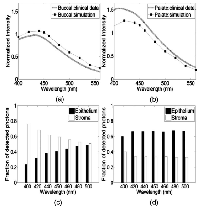
Fig. 4 Comparison of Monte Carlo model predictions with clinical fluorescence spectra measured at different anatomic sites in the oral cavity. Clinical data and predictions at 350-nm excitation from (a) normal buccal mucosa and (b) normal palate. Bar graphs showing the predicted fraction of detected photons originating from the epithelium and stroma for (c) normal buccal mucosa and (d) normal palate.
