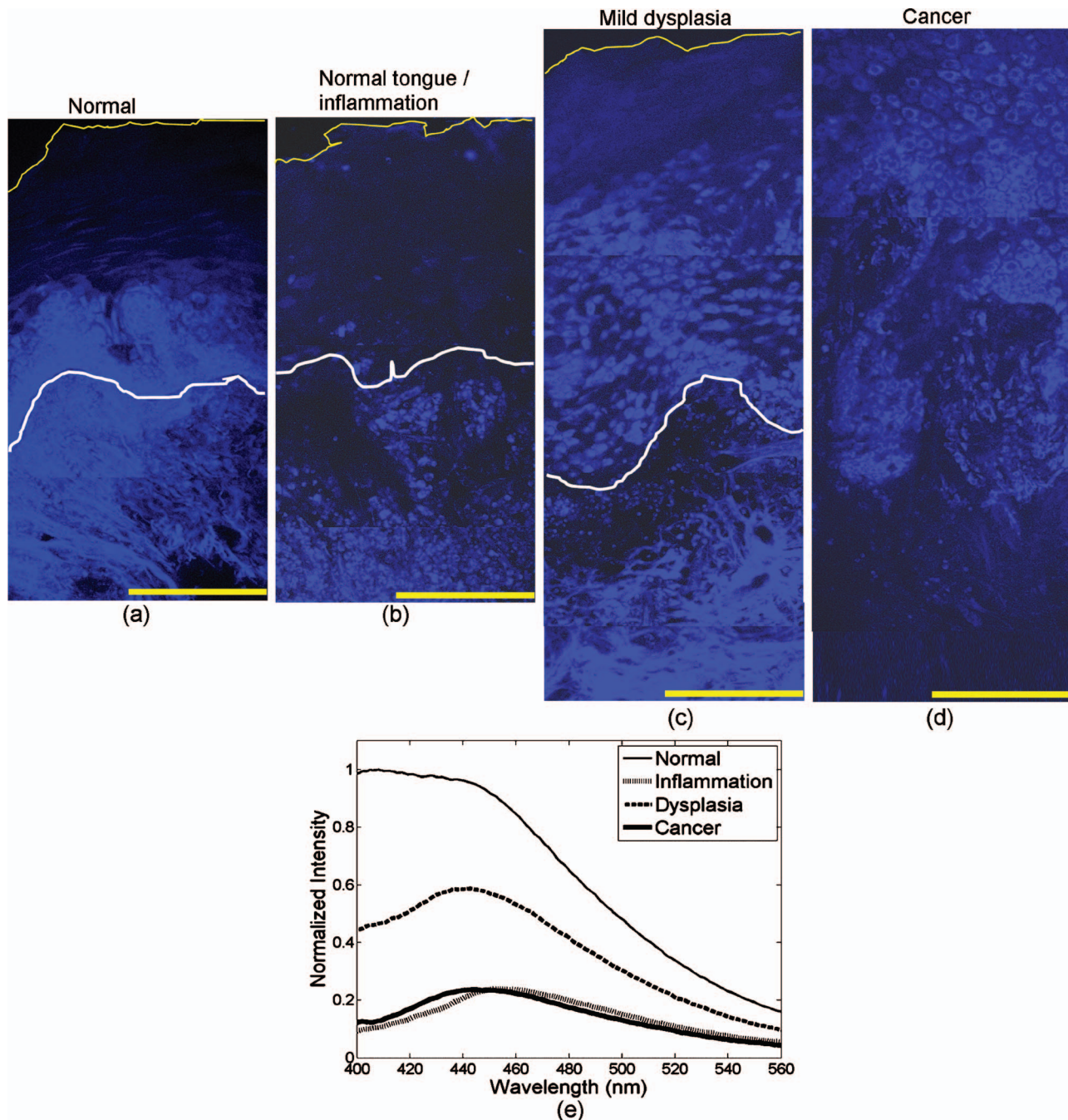
Fig. 1 (a) to (d) Fluorescence confocal images and (e) measured fluorescence spectra at UV excitation, showing neoplastic progression in the tongue. (a) Normal tongue; (b) normal tongue with severe stromal inflammation; (c) focal mild dysplasia; and (d) moderately differentiated cancer. In (a), (b), and (c), the white lines represent the basement membrane and the yellow lines represent the tissue surface. Scale bars represent 200 \mu\text{m} . (e) Fluorescence spectra at 350-nm excitation, measured from the same oral sites shown in the confocal images. Images (b) and (c) are reproduced from Ref. 6 with permission.
