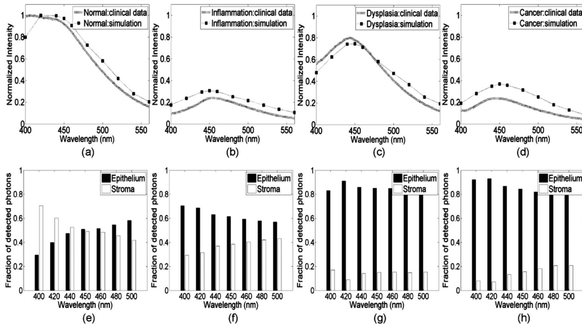
Fig. 2 Comparison of Monte Carlo model predictions with clinical fluorescence spectra measured from four oral tongue sites in the same patient. Clinical data and predictions at 350-nm excitation from (a) normal tongue, (b) normal tongue with severe inflammation, (c) focal mild dysplasia, and (d) moderately differentiated cancer. Bar graphs showing the predicted fraction of detected photons originating from the epithelium and the stroma for the (e) normal, (f) inflammatory, and (g) dysplastic simulations. (h) Bar graph showing the predicted fraction of detected photons originating from the cellular region (upper 400 \mu\text{m} , labeled as epithelium on the bar graph) and the deeper fibrous regions (labeled as stroma on the bar graph) for the cancer simulation.
