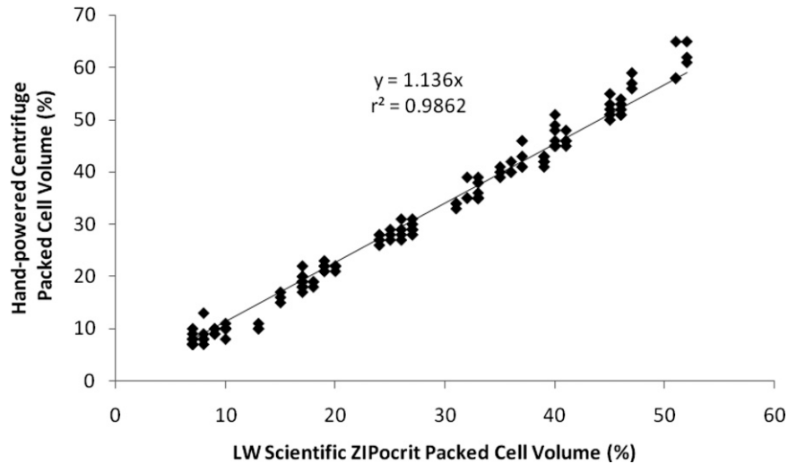
FIGURE 3. Measurement of packed cell volume (PCV) by using the hand-powered centrifuge with a 10-minute pumping time versus reference values determined by using the ZIPocrit centrifuge with a five-minute spin time. The PCV determined by using the hand-powered centrifuge is approximately 14% higher than that measured with the ZIPocrit for all tested degrees of anemia.
