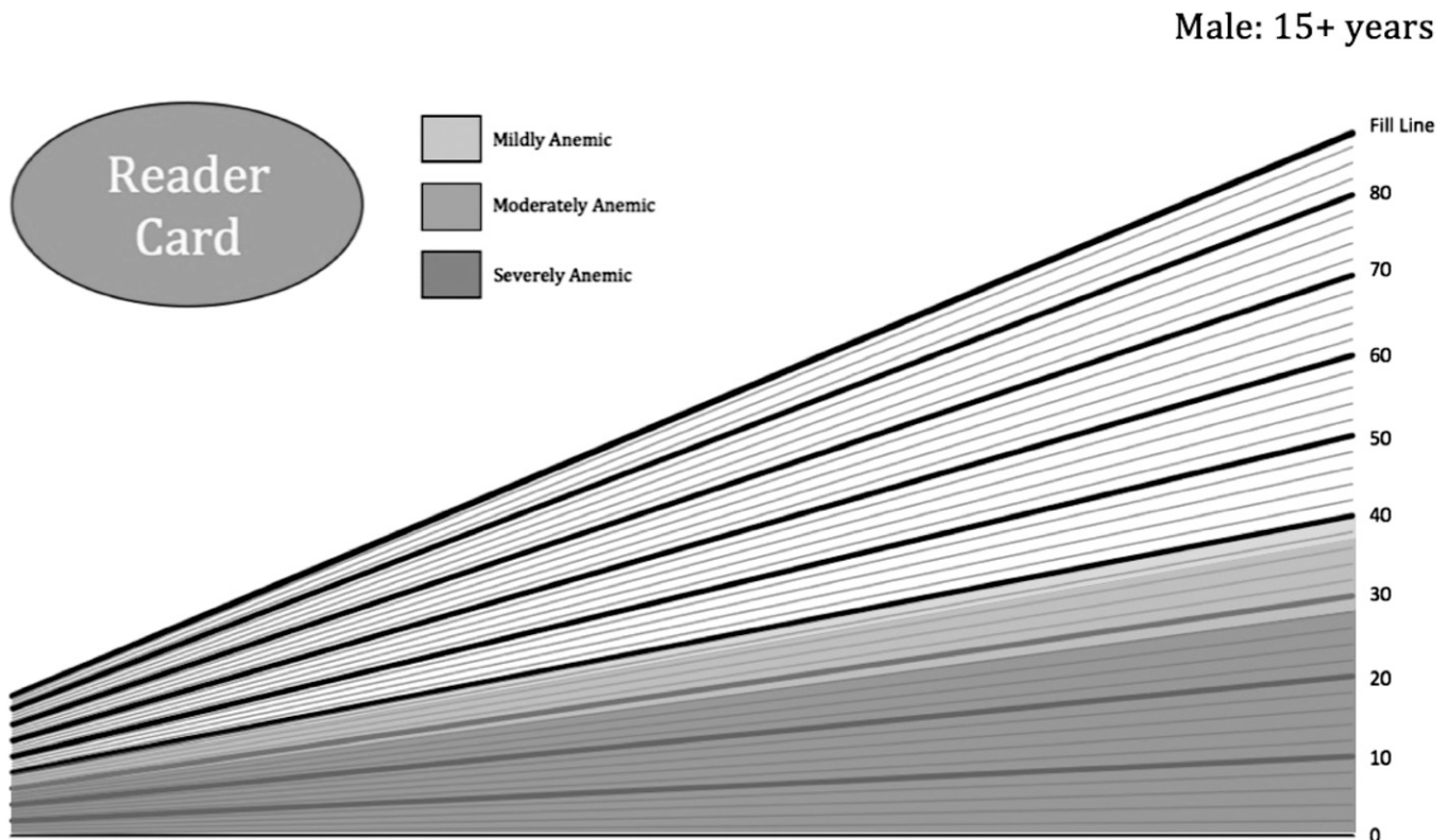
FIGURE 4. Adapted reader card for the hand-powered centrifuge. The slope of the lines converting packed cell volume to hematocrit are 1.14 times the slope of the lines on the standard reader cards on the basis of the calibration determined in Figure 3.
