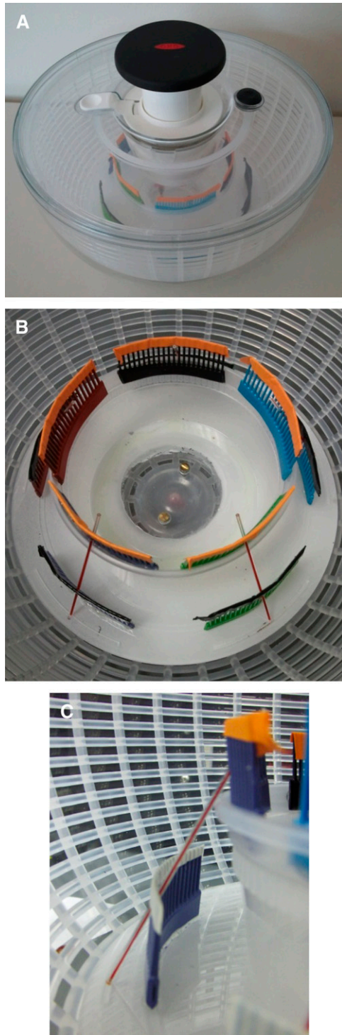
FIGURE 1. Hand-powered centrifuge: A , exterior; B , interior; and C , front view of microcapillary tube holder.
